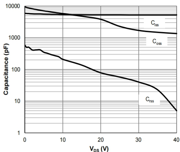
Figure 8: Capacitance Characteristics
