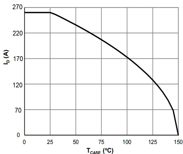
Figure 9: Current De-rating
