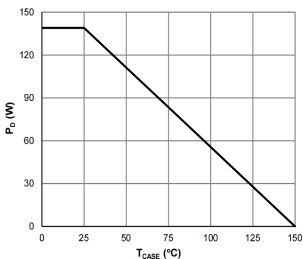
Figure 10: Power De-rating
